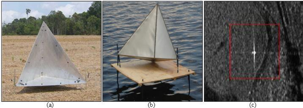
Figure 1 - Reflector installed in (a) an ideal place and (b) an aquatic platform and (c) example of a typical signal of a reflector in a SAR image.
