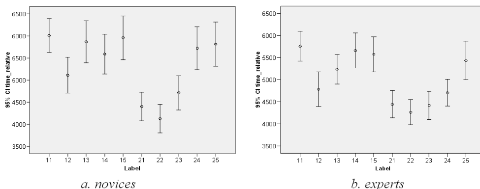
Figure 2: Error bars with a 95% confidence interval for the time intervals (ms) for locating subsequent labels
